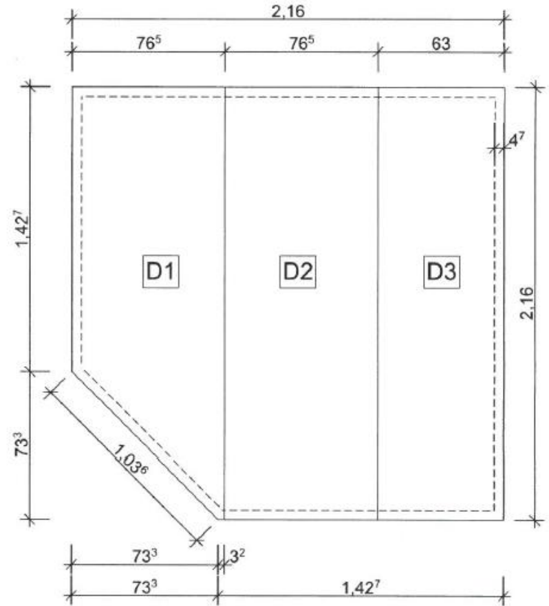
Roof element plan
